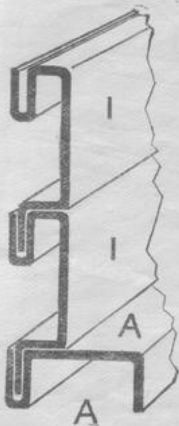
Double size illustration of a section showing the principle of construction.
