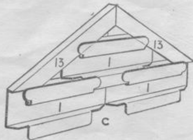
Elevation C. Interior of top wall, showing the fixing of the Cornice.
