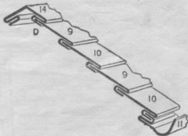
Section D shows Ridge Tile No. 14, with alternate rows of Slates No. 9, and Half Slates No. 10. Gutter No. 11 is attached to the last row of slates
